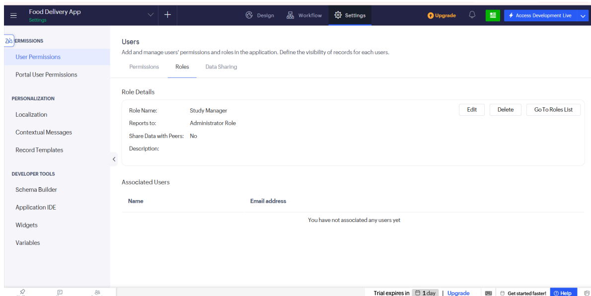
Figure 6: Study Manager permission configuration and user assignment.
