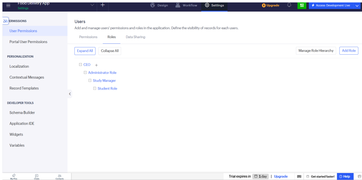
Figure 7: User and role hierarchy displayed in the Users section.
